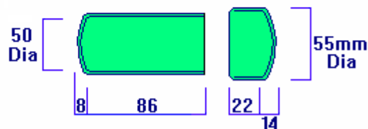
SECTIONAL ELEVATION
